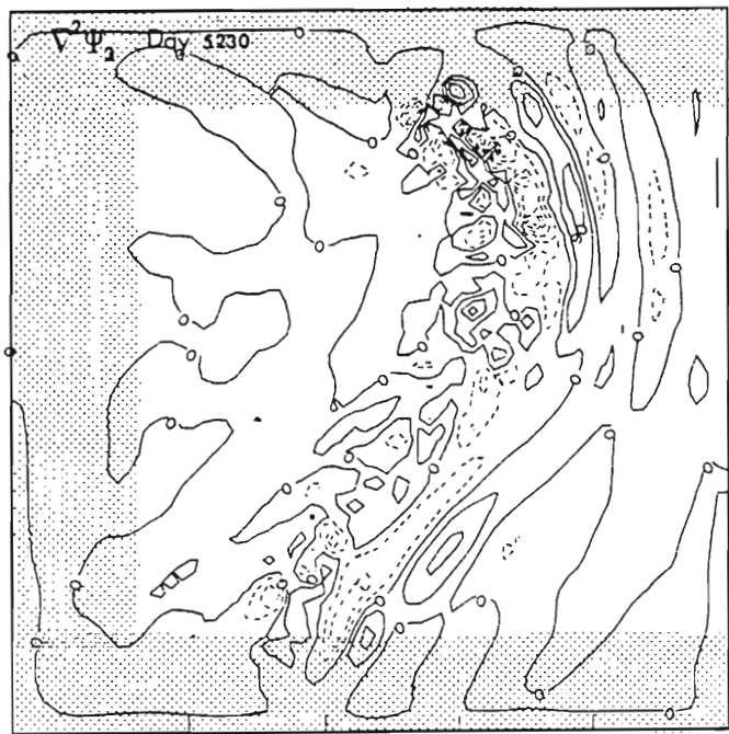
Figure 21. Ridge case. Instantaneous maps of the upper (top) and lower (bottom) vorticity field at day 5230. (March 30, year 15). Sponge layers are shaded. The ridge is a source of vorticity in both layers. Notice the baroclinic planetary waves in the western basin and the barotropic one in the eastern basin. Contour interval is 0.45 \times 10^{-7} \text{ sec}^{-1} .
