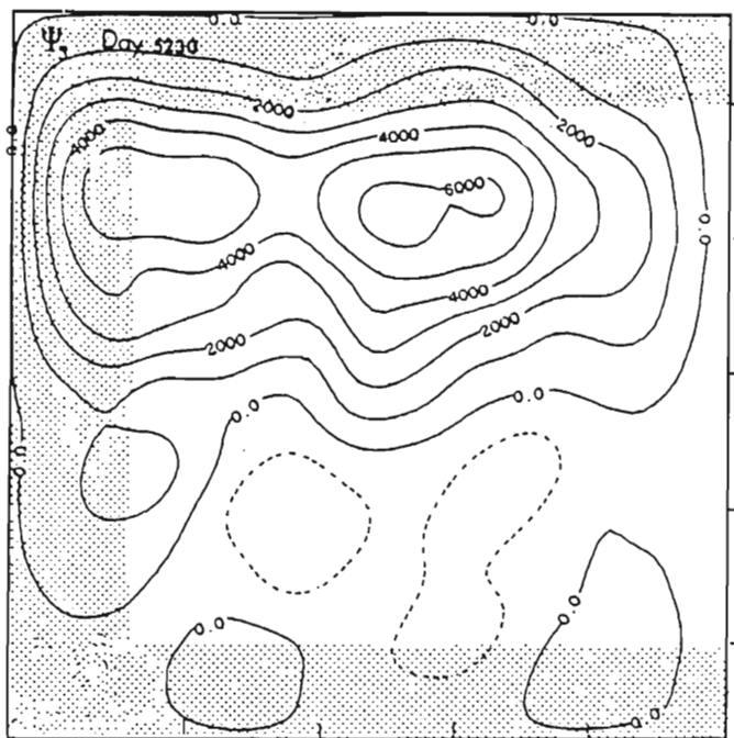
Figure 8. Flat bottom case. Instantaneous maps of the upper layer (top) and lower layer (bottom) streamfunctions. The picture is taken on March 30 in the 15 th year of simulation (Day 5230). The sponge regions are shaded. The patterns are barotropic at large scales whereas baroclinic features appear at lengthscales of about 500km. Contour interval is 1000\text{m}^2\text{sec}^{-1} .
